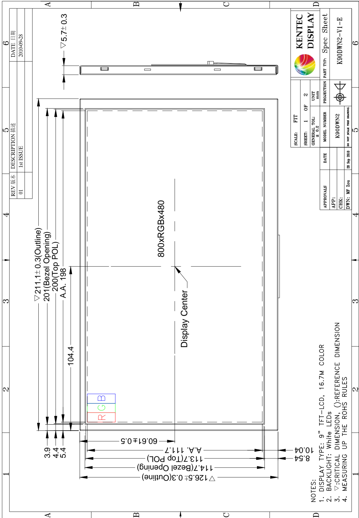
Figure 1-1: Outline Drawing 1
